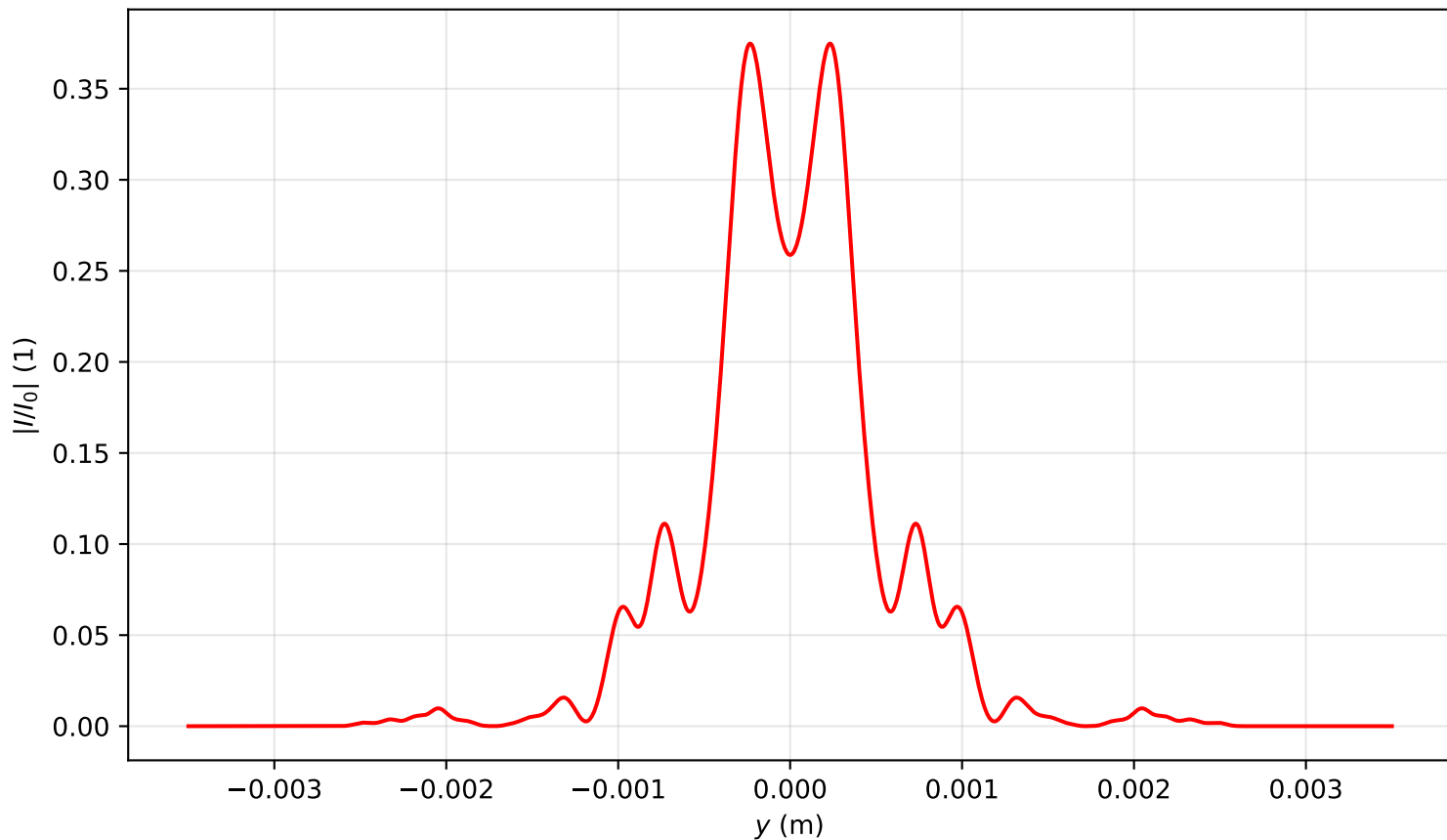
Intensity profile I(x=0, y, z=1.672)/I_0 , P_{in}=6.5P_{cr} , artificial time
